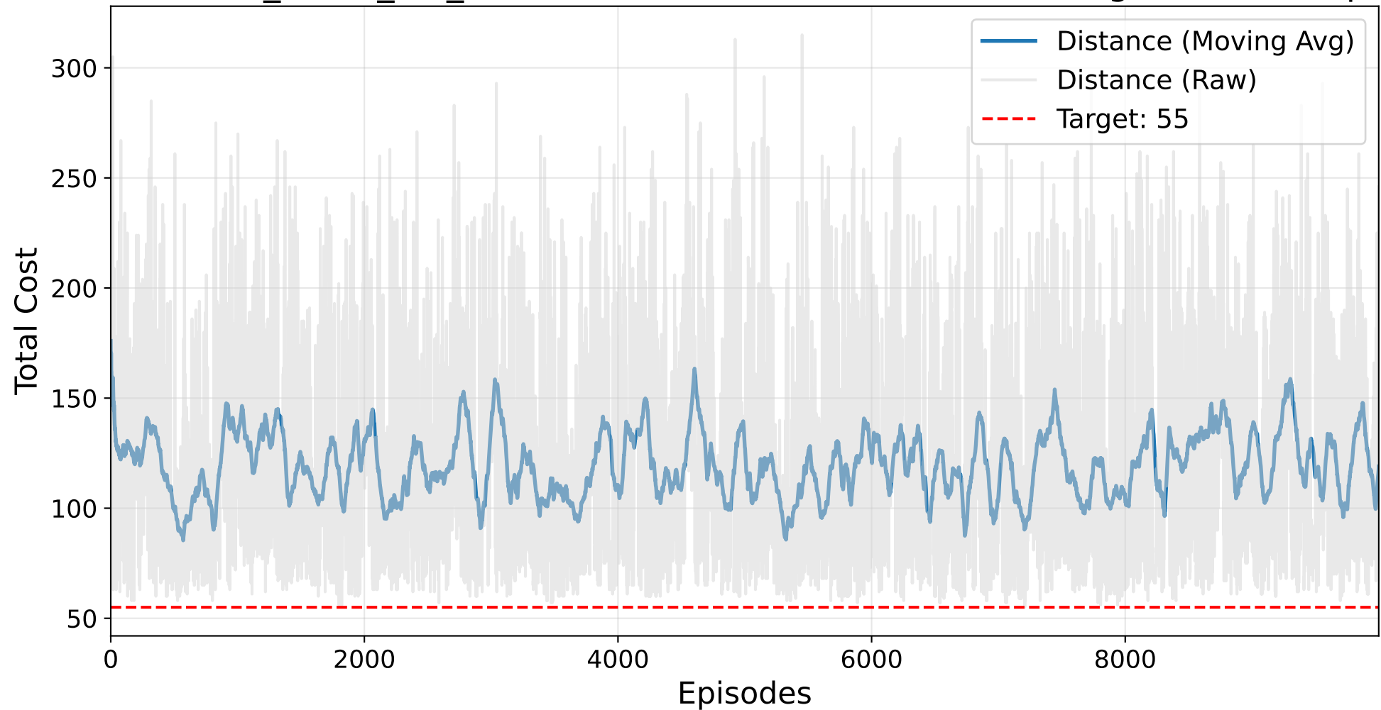
Final NO_MASK_NO_BAYESIAN Masked AutoRL-SOP Training - br17.12.sop
